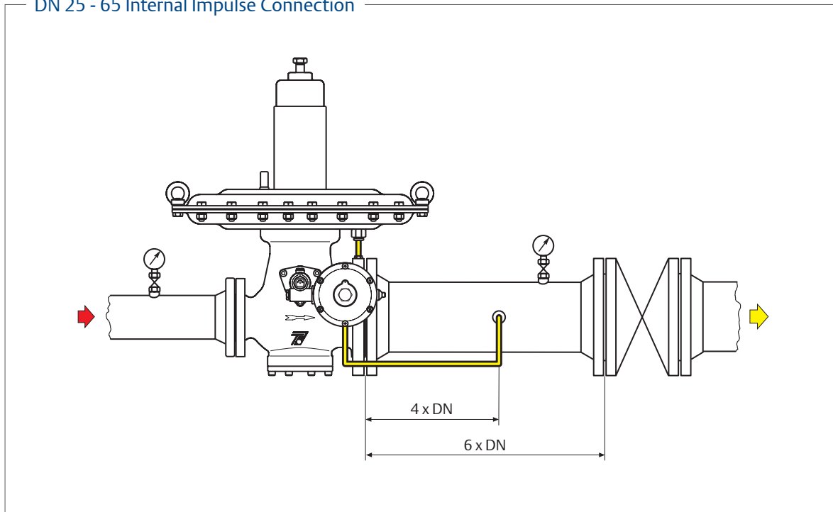
DN 25 - 65 Internal Impulse Connection
