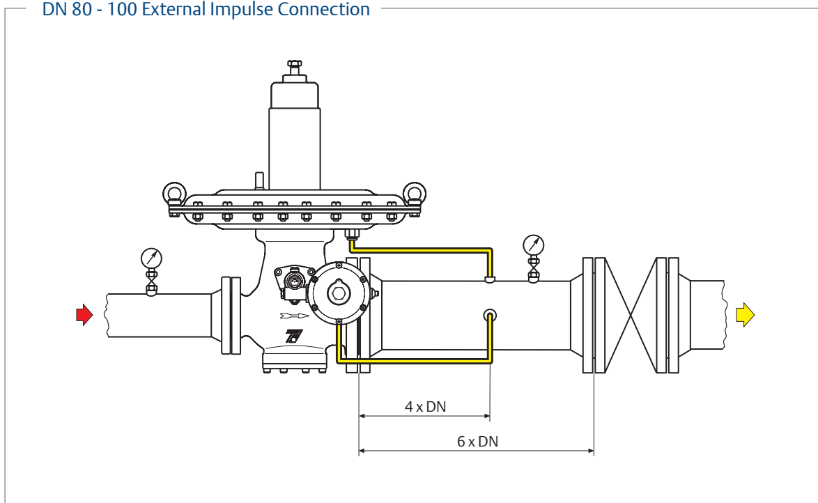
DN 80 - 100 External Impulse Connection
