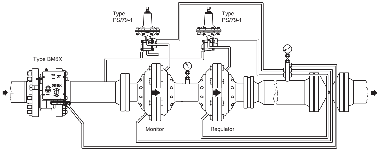
SLAM-SHUT VALVE WITH TYPE OS/80X-R CONTROLLER - INSTALLATION IN A LOW PRESSURE REGULATING LINE
