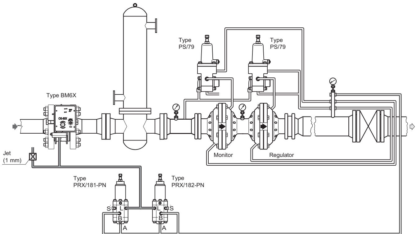
SLAM-SHUT VALVE WITH TYPE OS/80X-R-PN CONTROLLER - OVERPRESSURE AND UNDERPRESSURE CONTROL DOWNSTREAM OF REGULATORS
